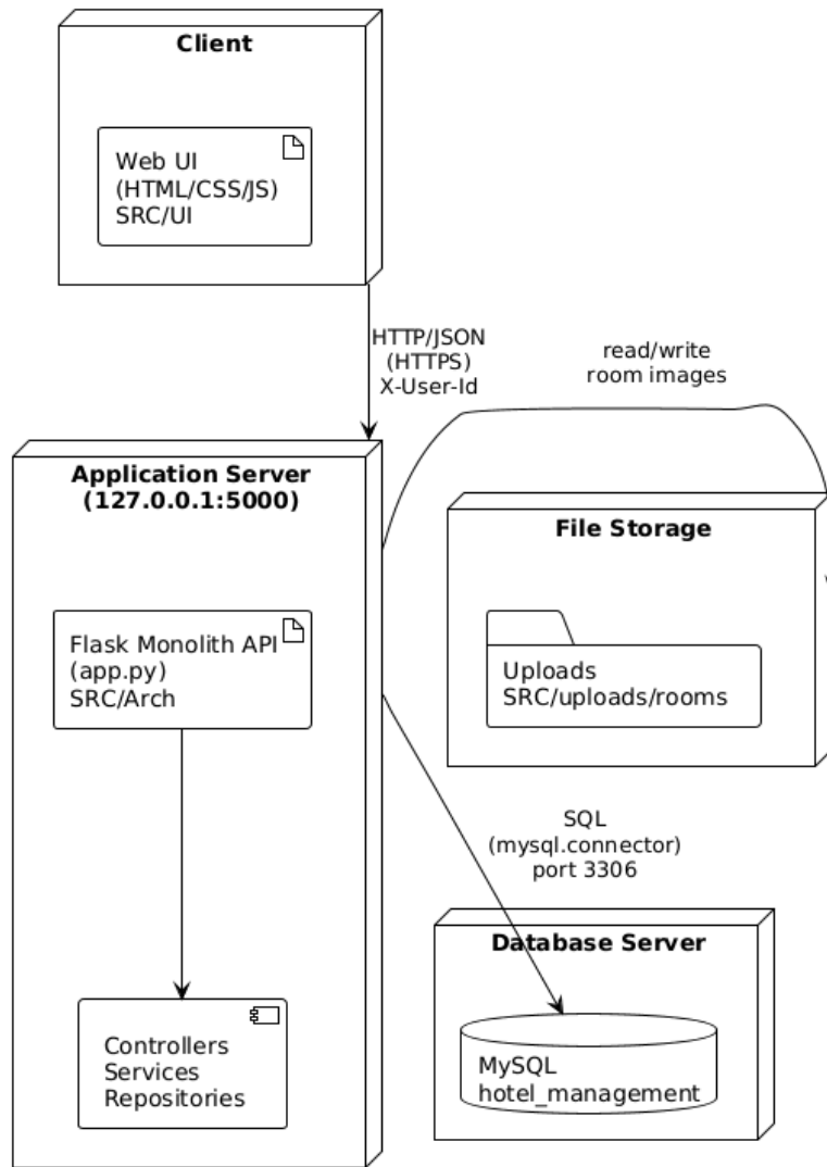
Figure 12: Deployment View
